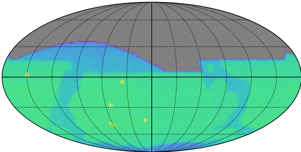
early_u_fpextra2.0_v3.4_10yrs z: CoaddM5
