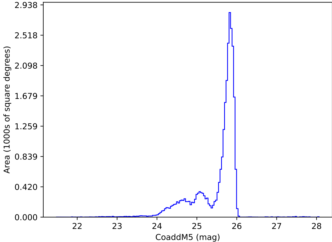
early_u_fpextra2.0_v3.4_10yrs z: CoaddM5
