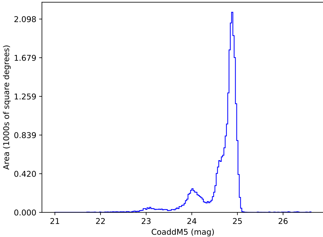
early_u_fpextra2.0_v3.4_10yrs y: CoaddM5
