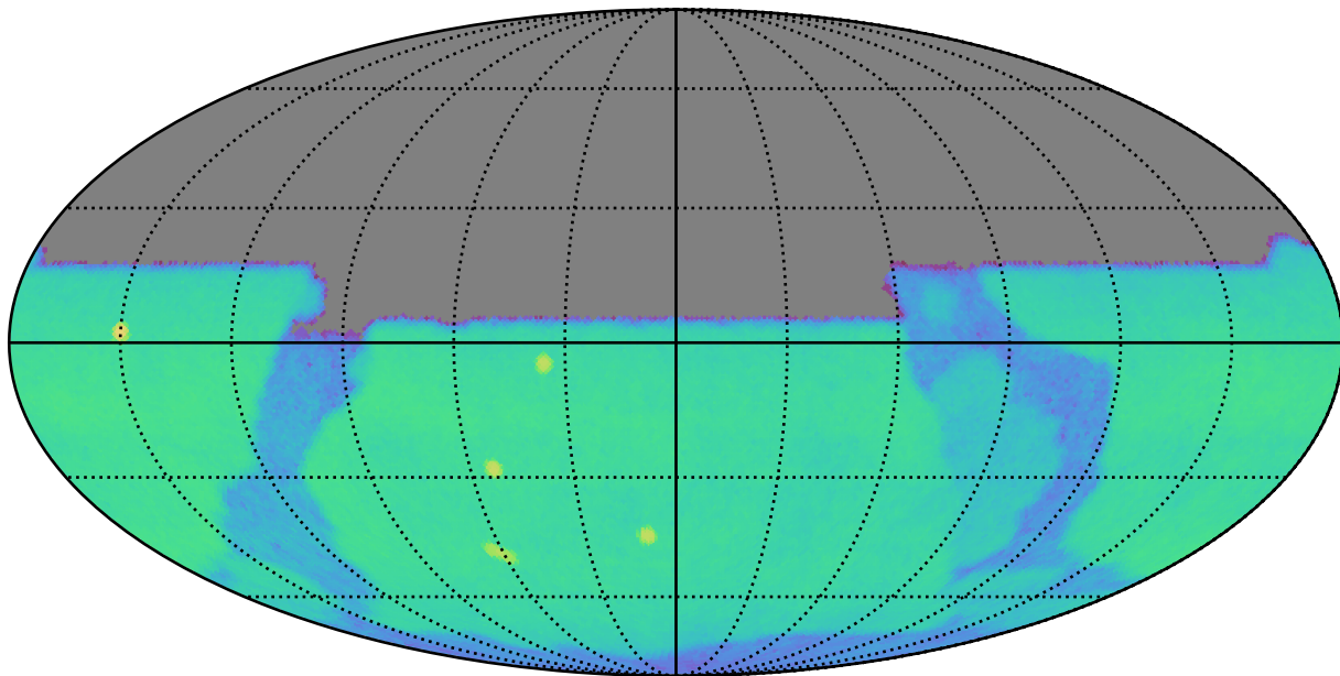
early_u_fpextra2.0_v3.4_10yrs u: CoaddM5
