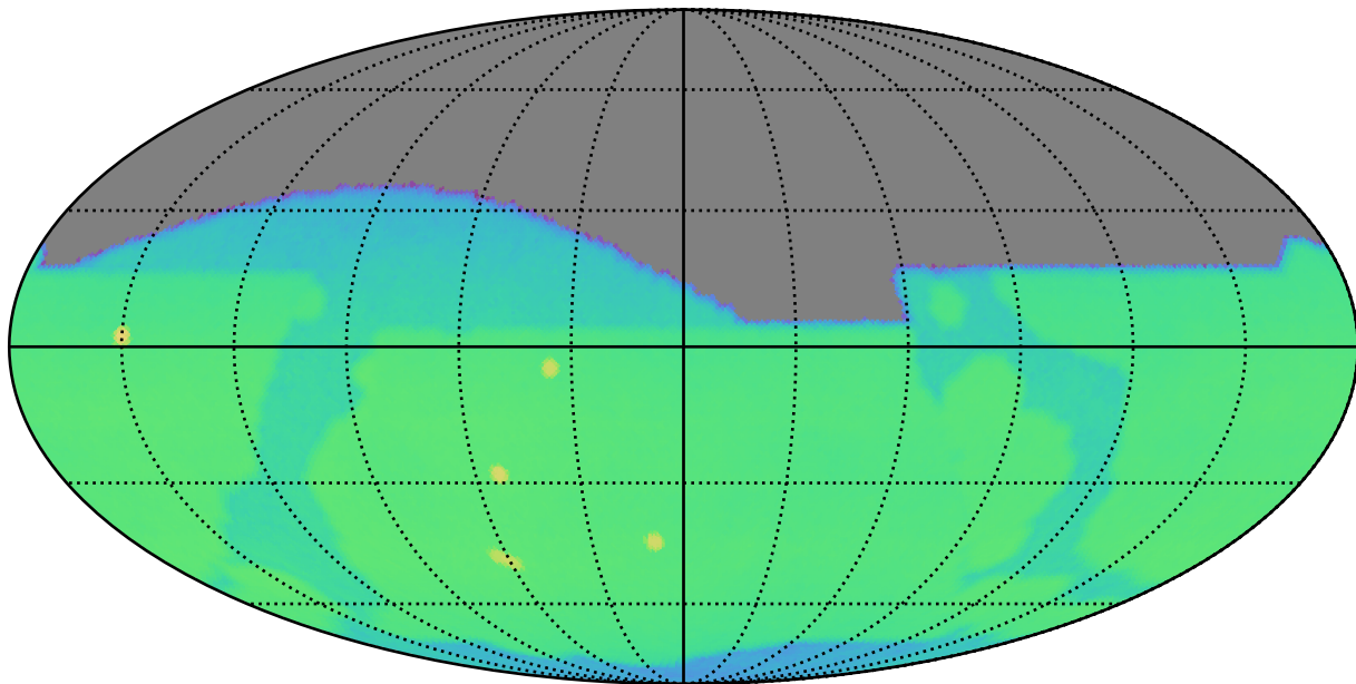
early_u_fpextra2.0_v3.4_10yrs r: CoaddM5
