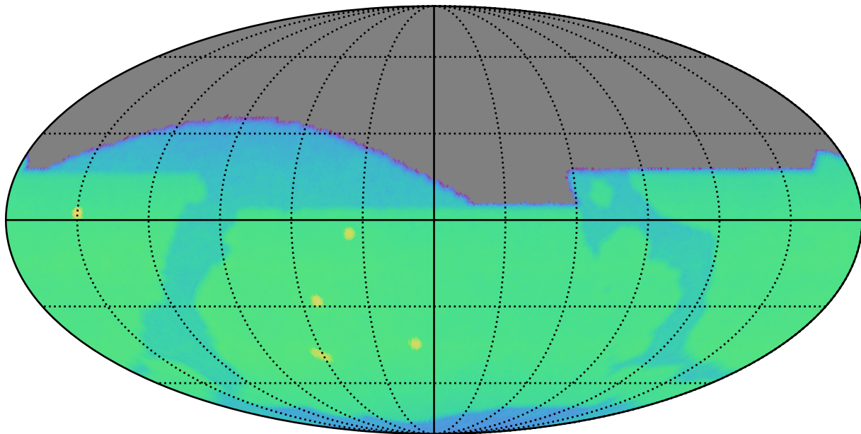
early_u_fpextra2.0_v3.4_10yrs i: CoaddM5
