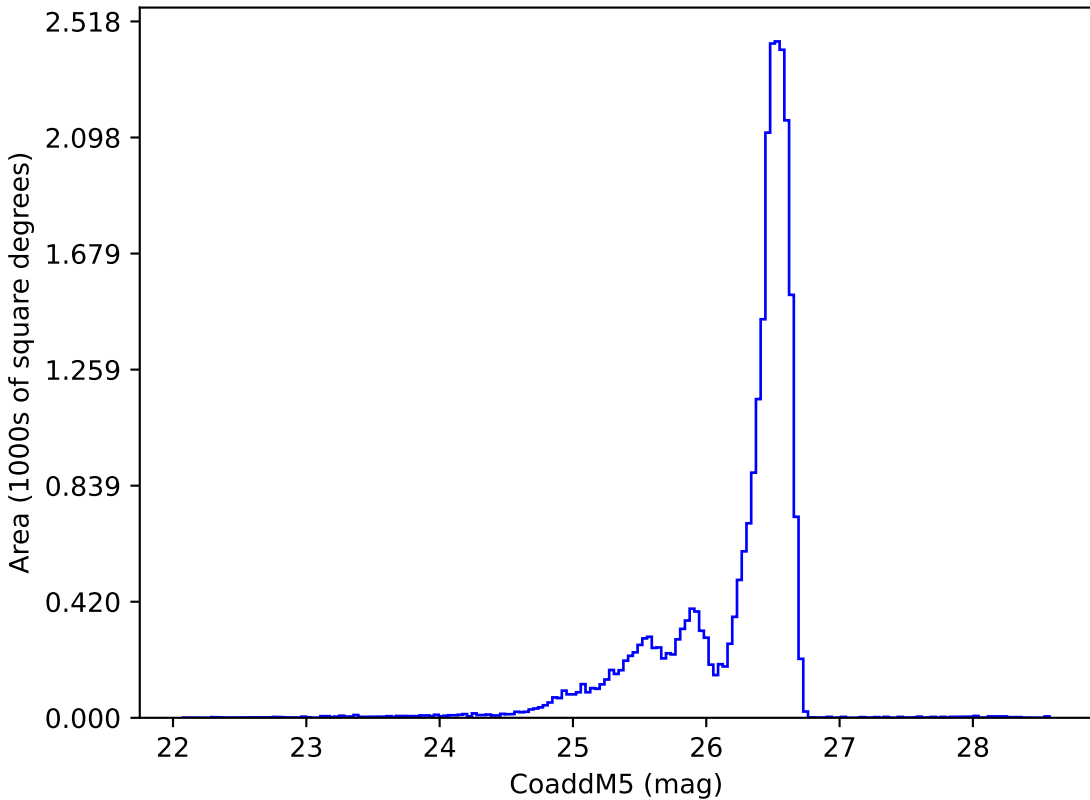
early_u_fpextra2.0_v3.4_10yrs i: CoaddM5
