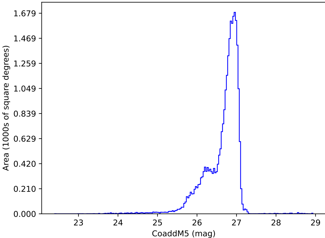
early_u_fpextra2.0_v3.4_10yrs g: CoaddM5
