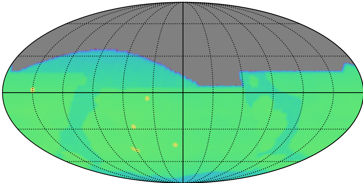
early_u_fpextra2.0_v3.4_10yrs : CoaddM5
