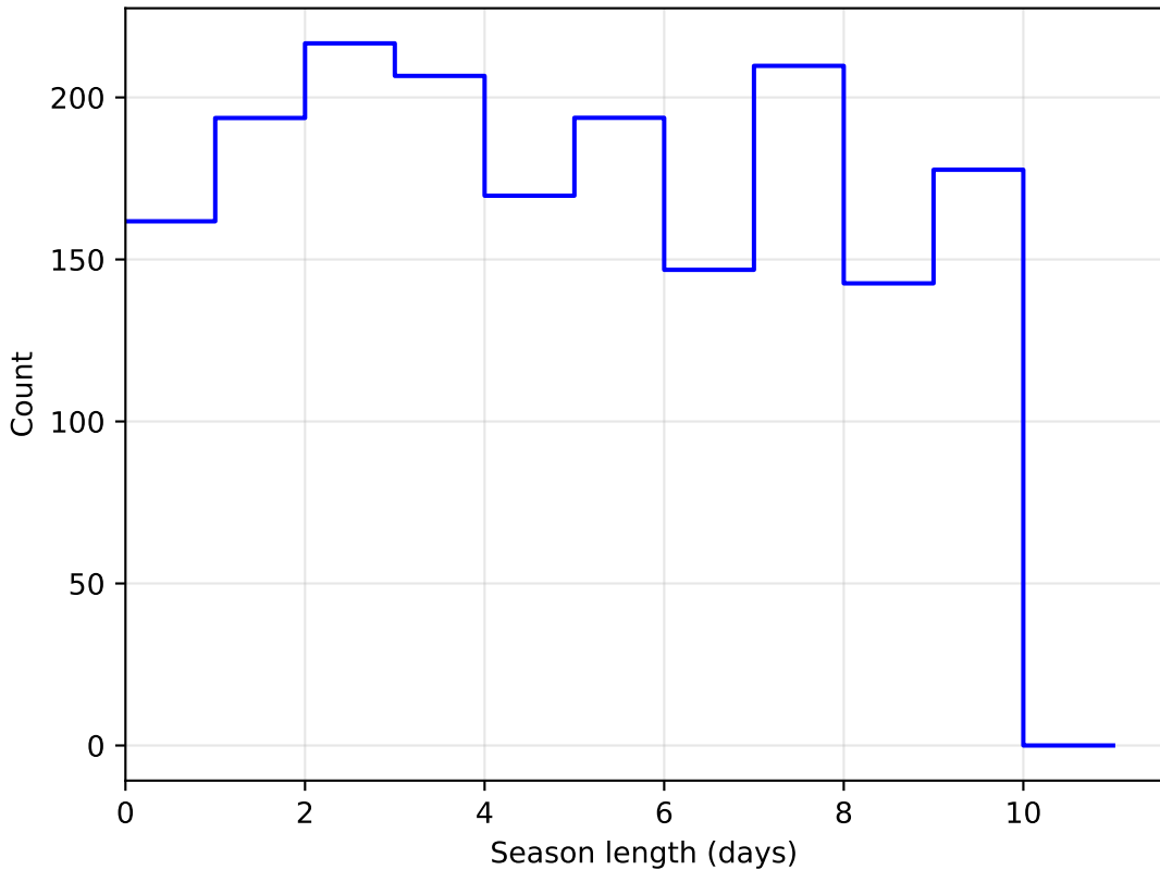
early_u_fpextra2.0_v3.4_10yrs DD:WFD all bands: SeasonLength
