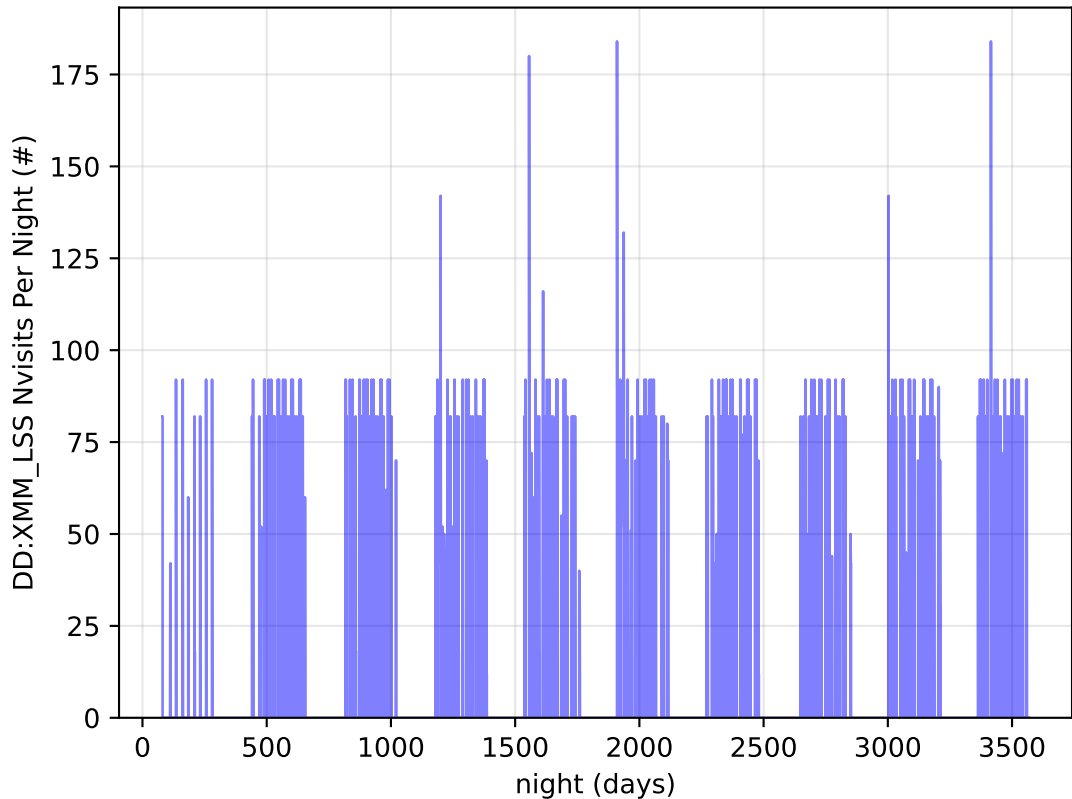
early_u_fpextra2.0_v3.4_10yrs all bands: DD:XMM_LSS Nvisits Per Night
