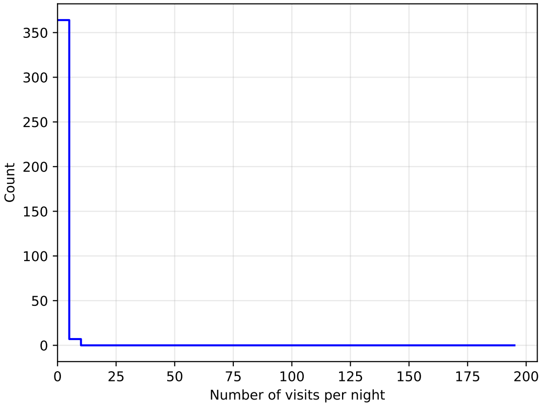
early_u_fpextra2.0_v3.4_10yrs all bands: DD:WFD NVisitsPerNight
