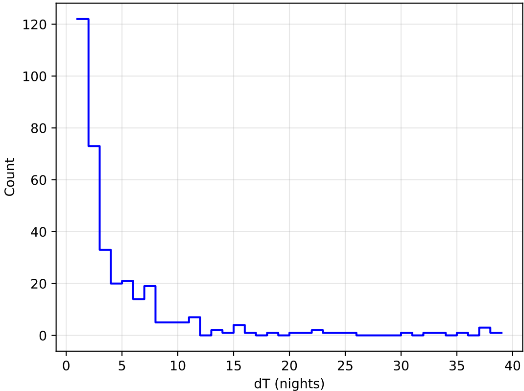
early_u_fpextra2.0_v3.4_10yrs all bands: DD:WFD Delta Nights Histogram
