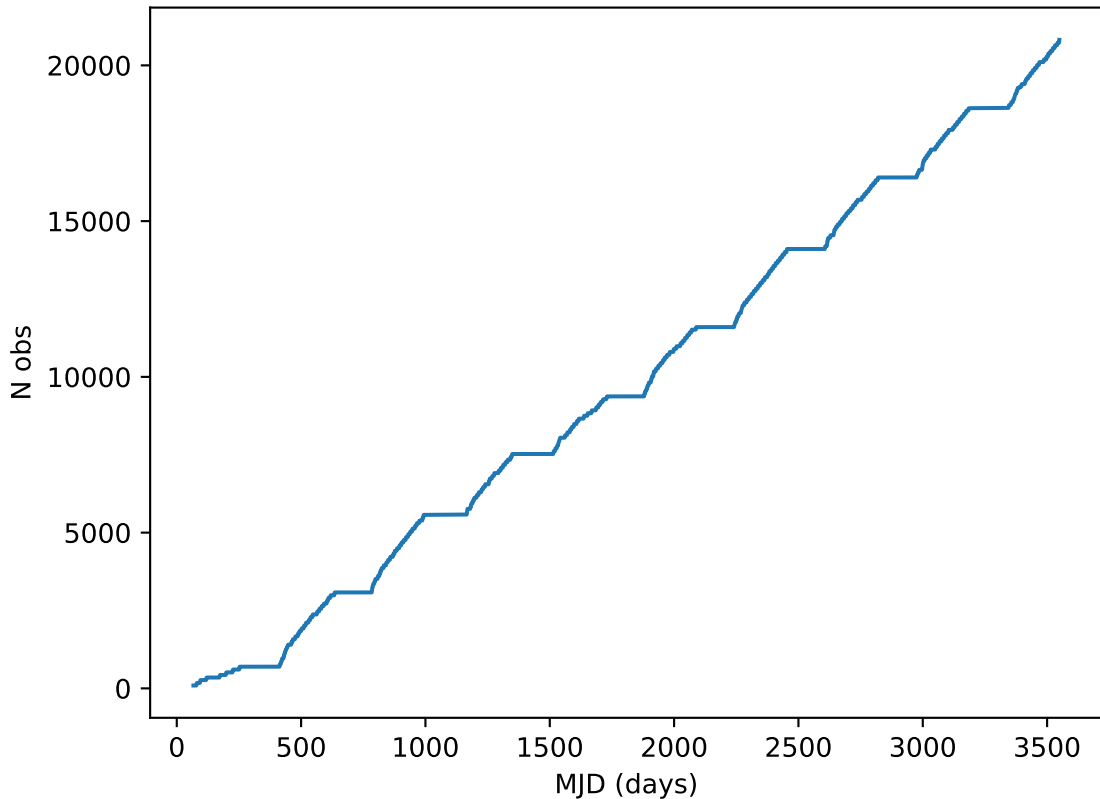
early_u_fpextra2.0_v3.4_10yrs all bands: DD:ELAISS1 Cumulative NVisits
