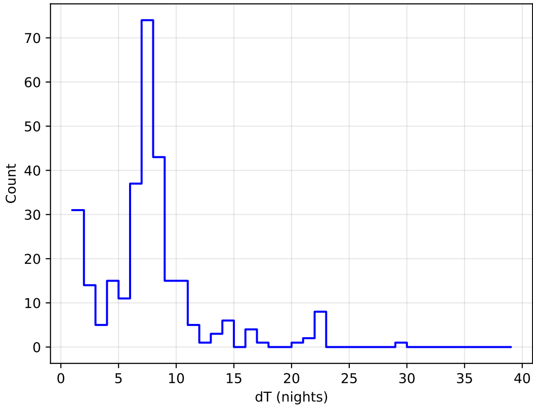
early_u_fpextra2.0_v3.4_10yrs all bands: DD:EDFS Delta Nights Histogram
