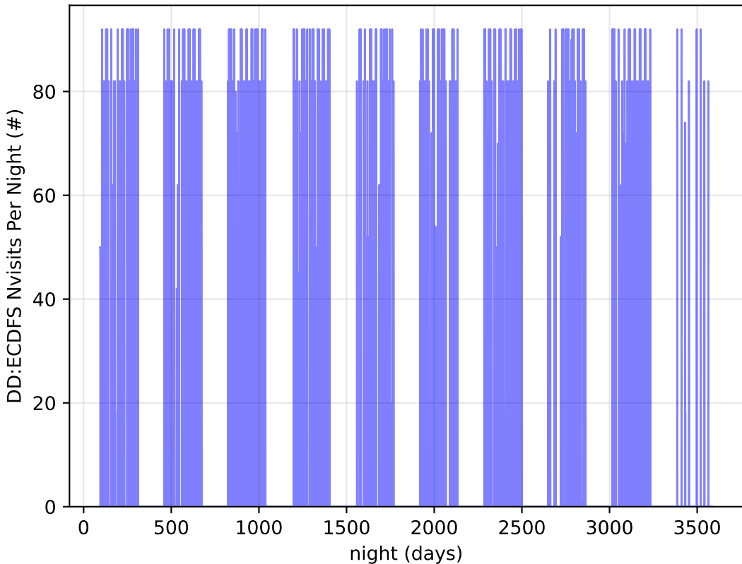
early_u_fpextra2.0_v3.4_10yrs all bands: DD:ECDFS Nvisits Per Night
