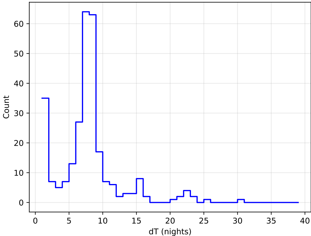
early_u_fpextra2.0_v3.4_10yrs all bands: DD:ECDFS Delta Nights Histogram
