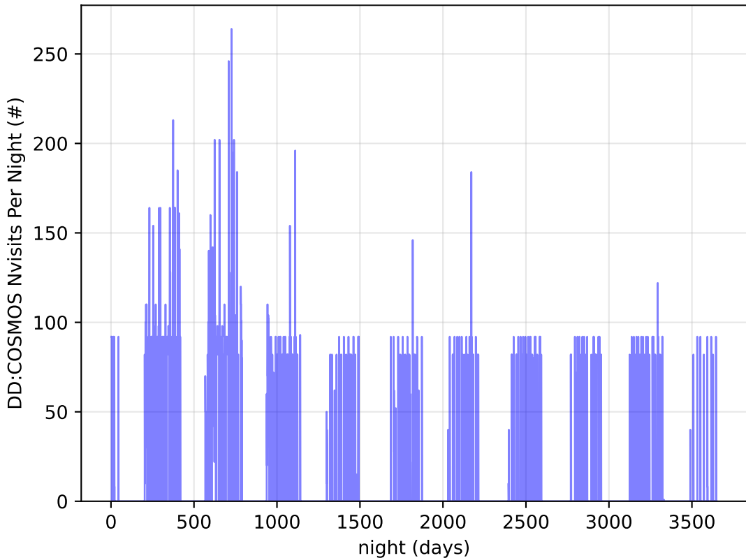
early_u_fpextra2.0_v3.4_10yrs all bands: DD: COSMOS Nvisits Per Night
