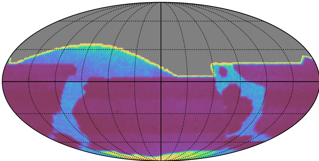
early_ss_template_fpextra5.0_v3.4_10yrs : properMotion
