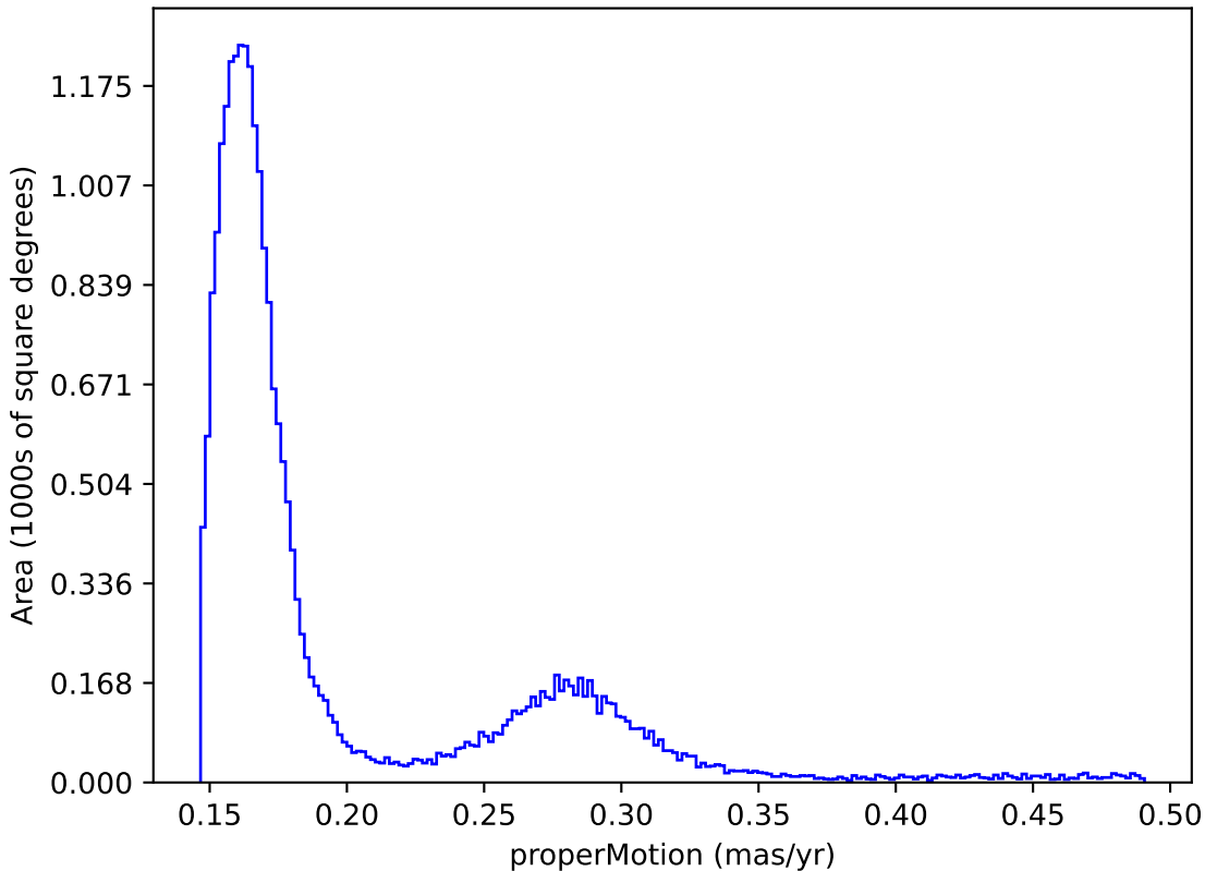
early_ss_template_fpextra5.0_v3.4_10yrs : properMotion
