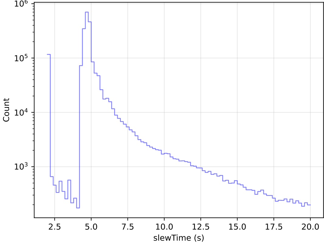
early_ss_template_fpextra5.0_v3.4_10yrs All visits: Zoom Slew Time Histogram
