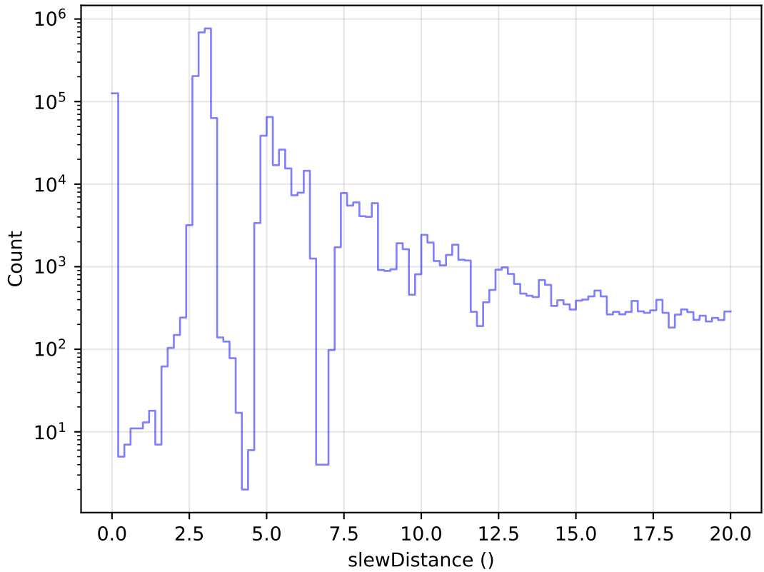
early_ss_template_fpextra5.0_v3.4_10yrs All visits: Zoom Slew Distance Histogram
