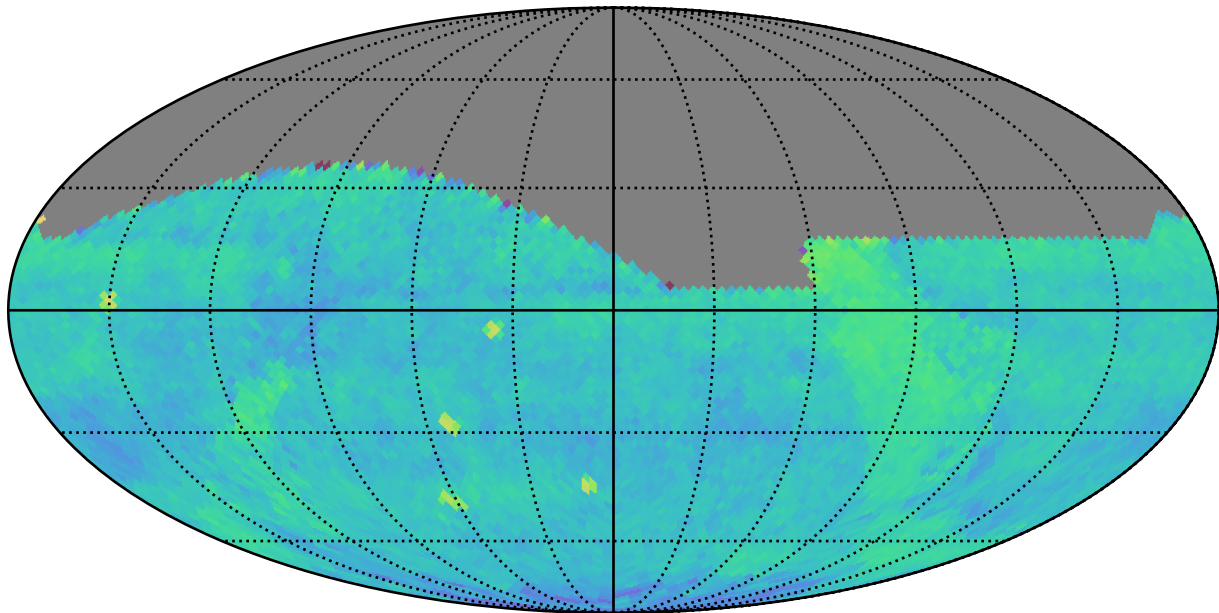
early_ss_template_fpextra5.0_v3.4_10yrs (g or r or i): PairFraction
