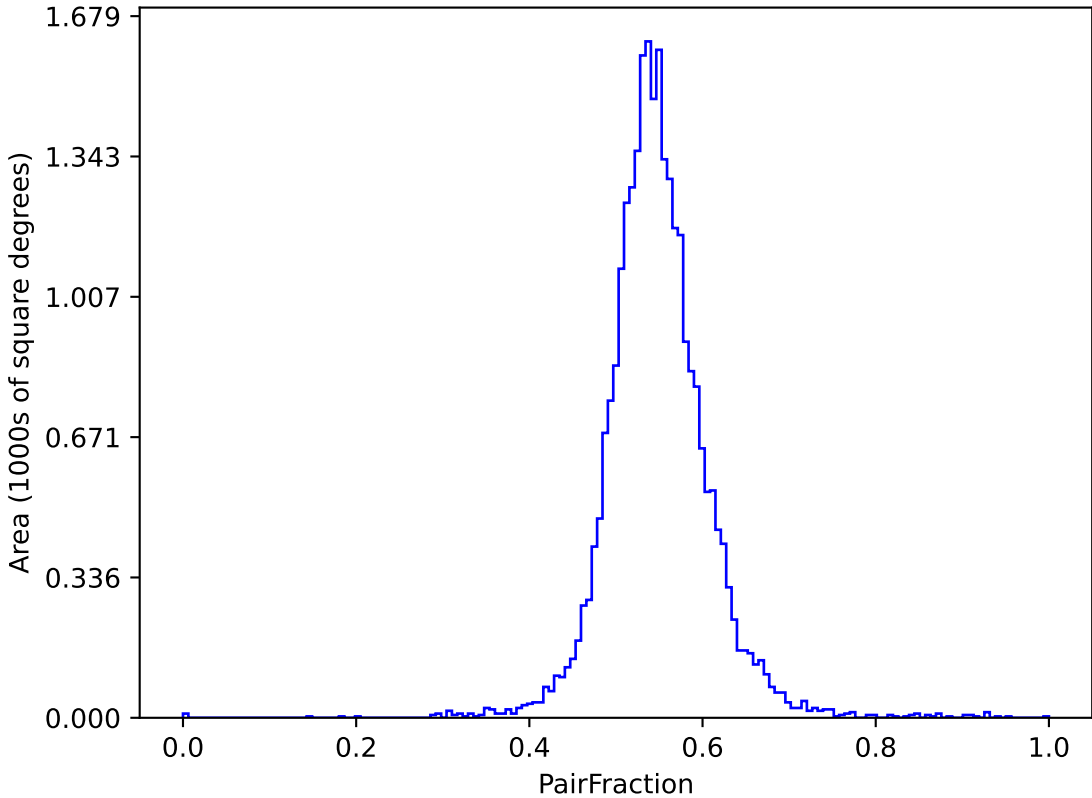
early_ss_template_fpextra5.0_v3.4_10yrs (g or r or i): PairFraction
