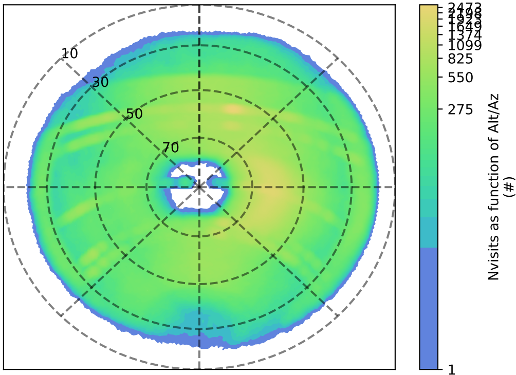
early_ss_template_fpextra5.0_v3.4_10yrs z: Nvisits as function of Alt/Az
