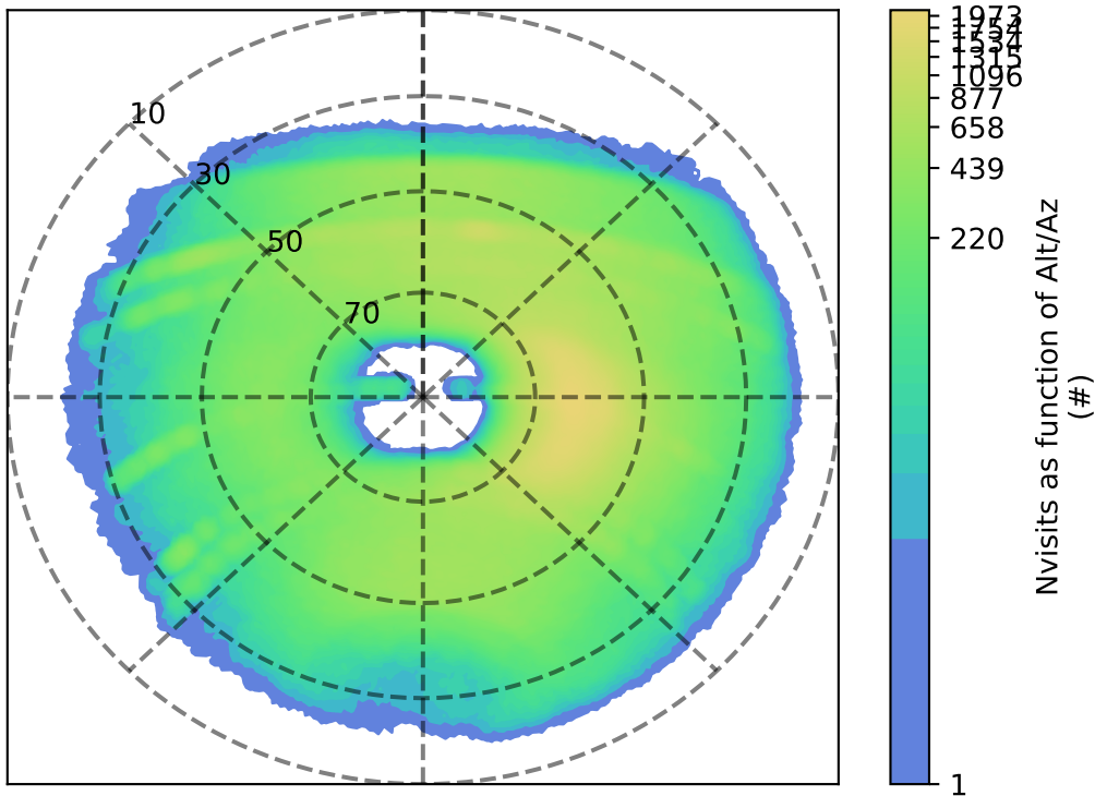
early_ss_template_fpextra5.0_v3.4_10yrs y: Nvisits as function of Alt/Az
