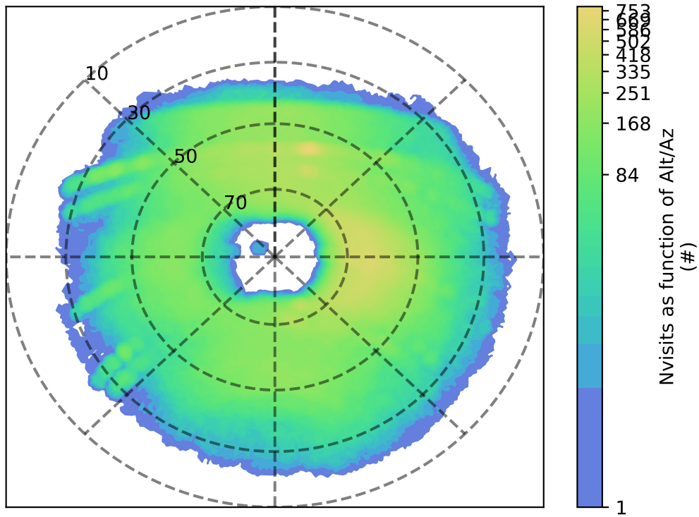
early_ss_template_fpextra5.0_v3.4_10yrs u: Nvisits as function of Alt/Az
