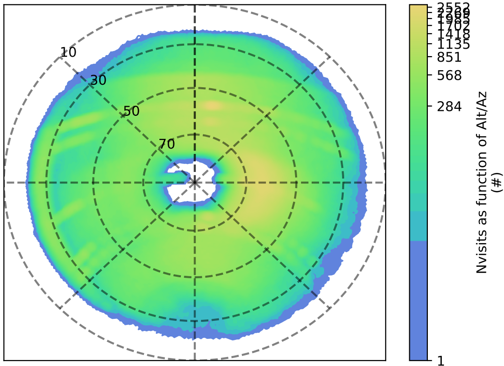
early_ss_template_fpextra5.0_v3.4_10yrs r: Nvisits as function of Alt/Az
