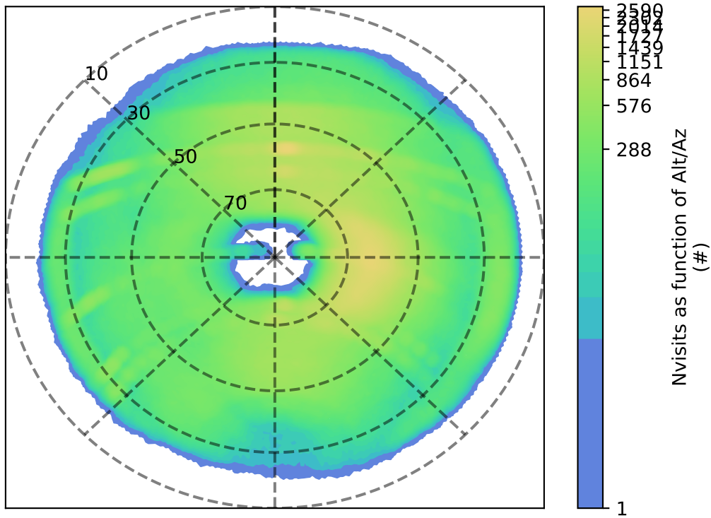
early_ss_template_fpextra5.0_v3.4_10yrs i: Nvisits as function of Alt/Az
