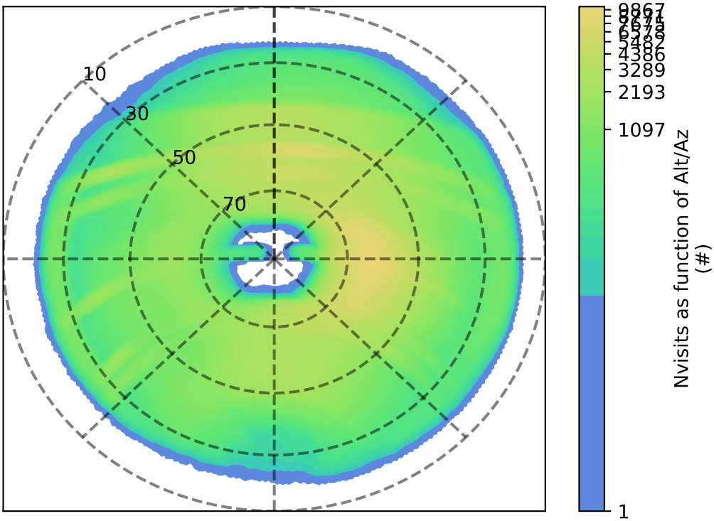
early_ss_template_fpextra5.0_v3.4_10yrs : Nvisits as function of Alt/Az
