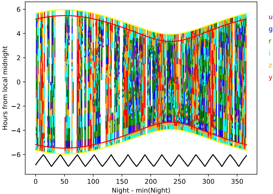
early_ss_template_fpextra5.0_v3.4_10yrs year 8-9: Hourglass
