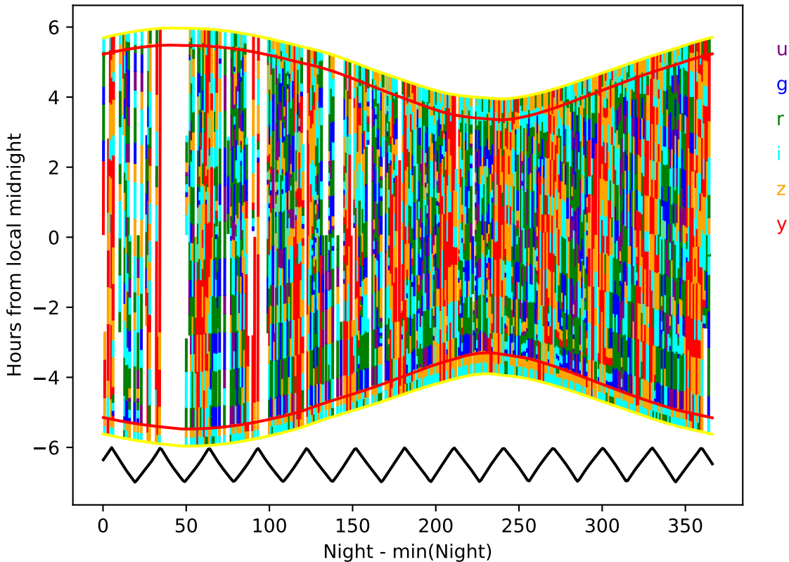
early_ss_template_fpextra5.0_v3.4_10yrs year 6-7: Hourglass
