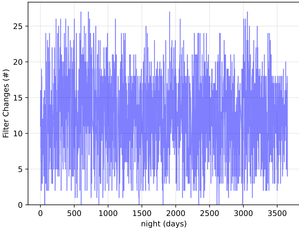
early_ss_template_fpextra5.0_v3.4_10yrs : Filter Changes
