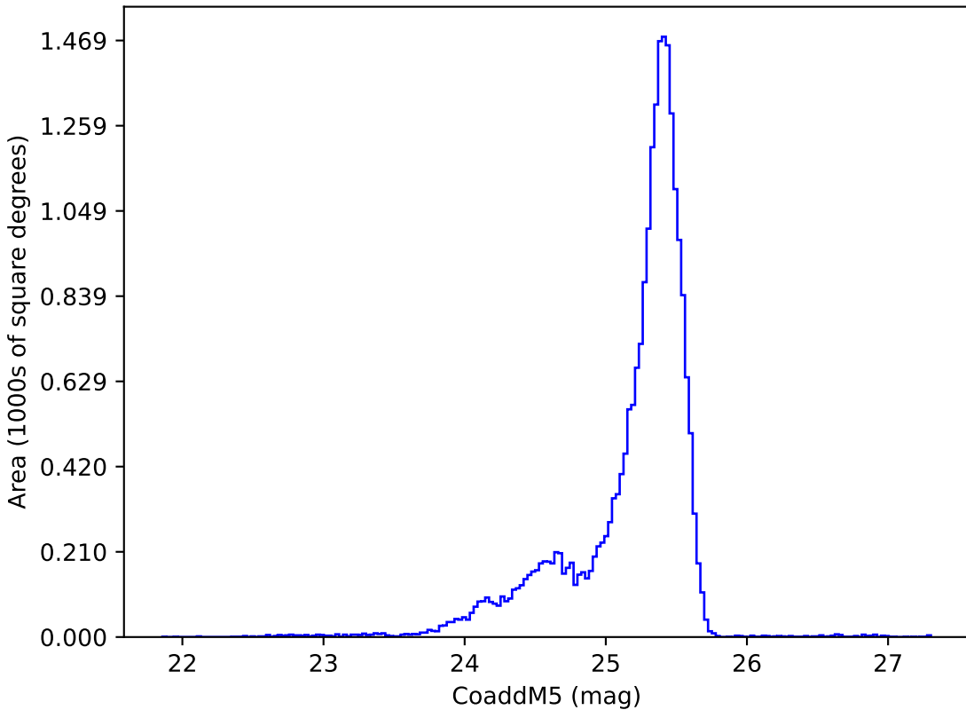
early_ss_template_fpextra5.0_v3.4_10yrs u: CoaddM5
