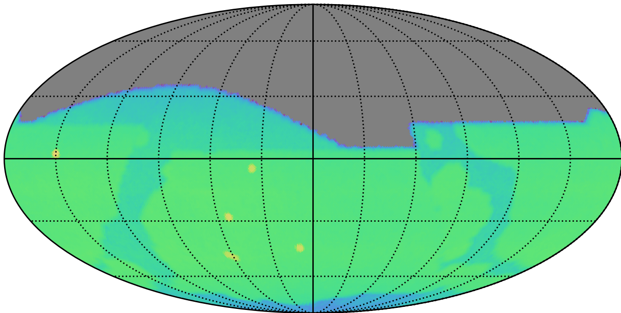
early_ss_template_fpextra5.0_v3.4_10yrs r: CoaddM5
