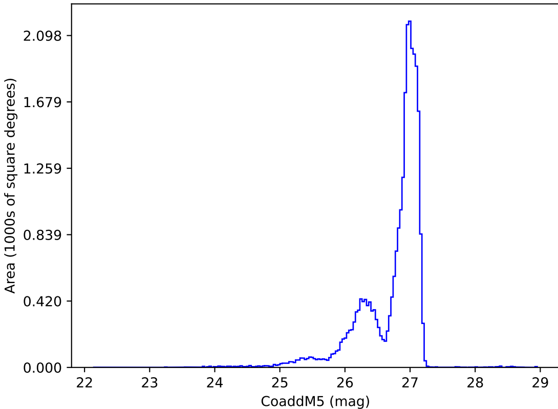
early_ss_template_fpextra5.0_v3.4_10yrs r: CoaddM5
