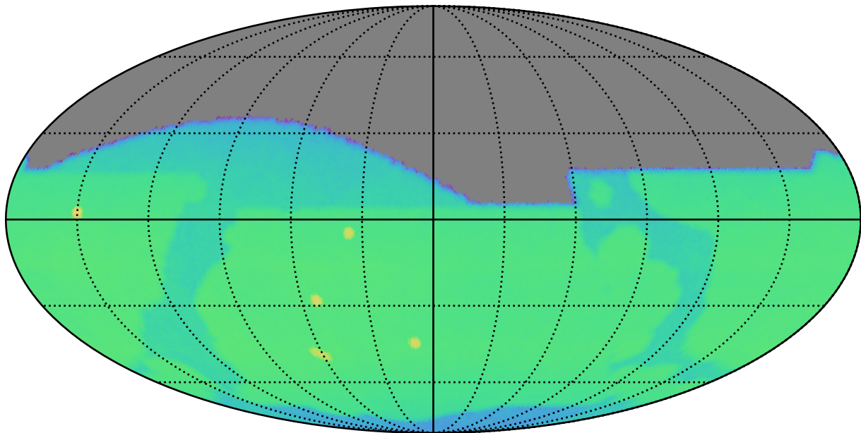
early_ss_template_fpextra5.0_v3.4_10yrs i: CoaddM5
