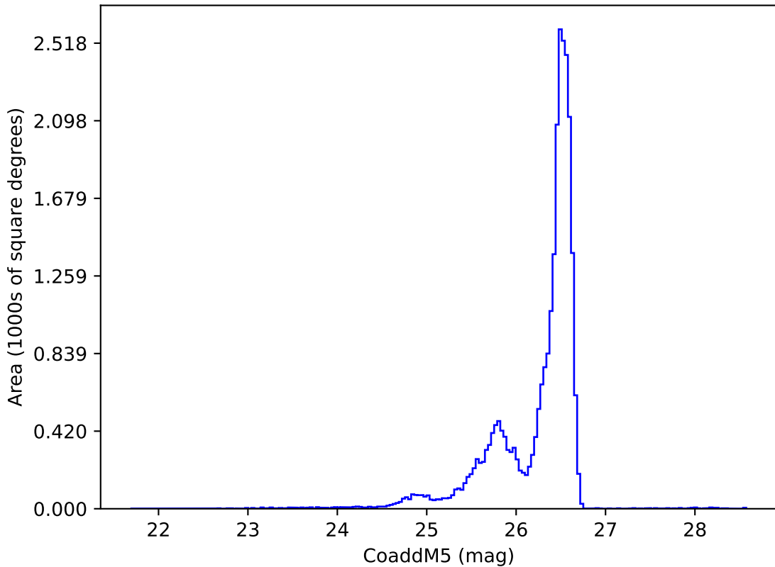
early_ss_template_fpextra5.0_v3.4_10yrs i: CoaddM5
