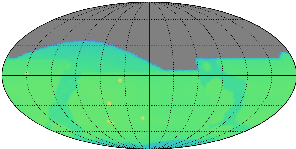
early_ss_template_fpextra5.0_v3.4_10yrs : CoaddM5
