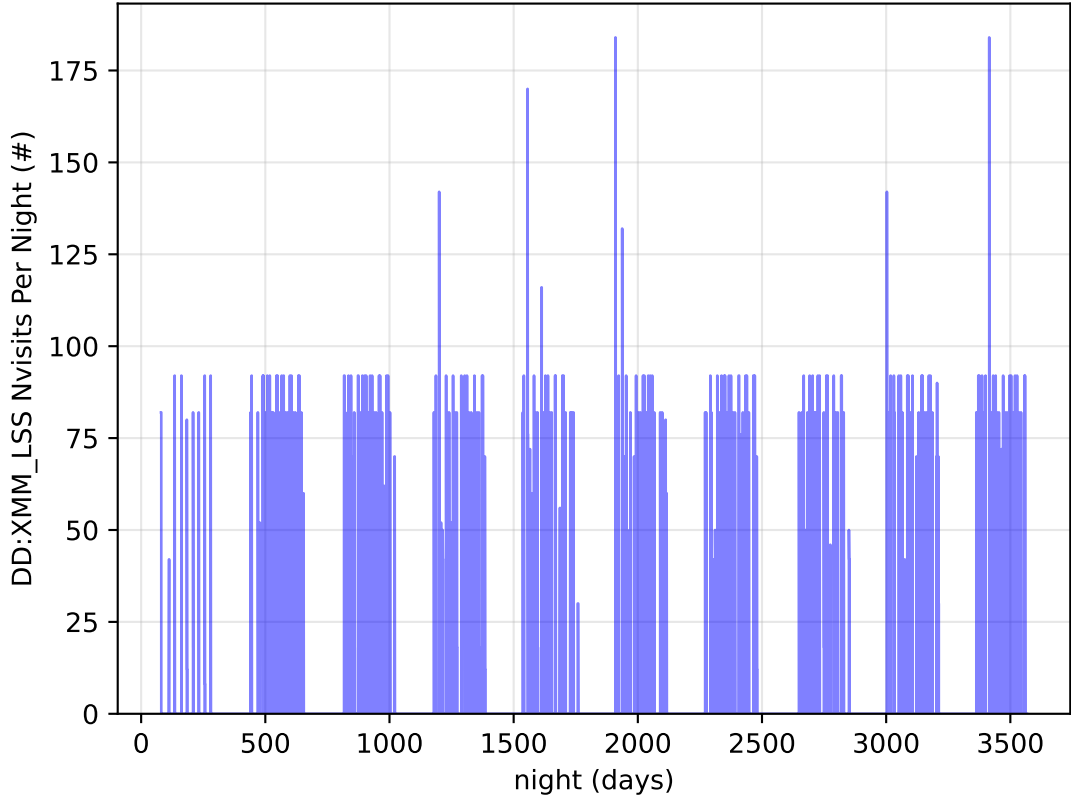
early_ss_template_fpextra5.0_v3.4_10yrs all bands: DD:XMM_LSS Nvisits Per Night
