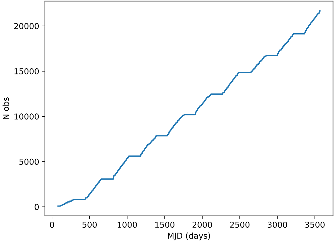
early_ss_template_fpextra5.0_v3.4_10yrs all bands: DD:XMM_LSS Cumulative NVisits
