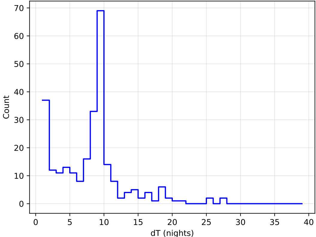
early_ss_template_fpextra5.0_v3.4_10yrs all bands: DD:ELAISS1 Delta Nights Histogram
