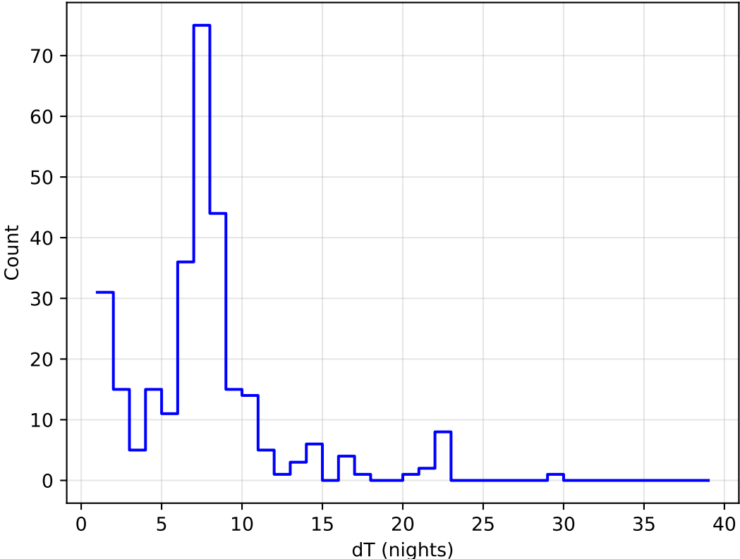
early_ss_template_fpextra5.0_v3.4_10yrs all bands: DD:EDFS Delta Nights Histogram
