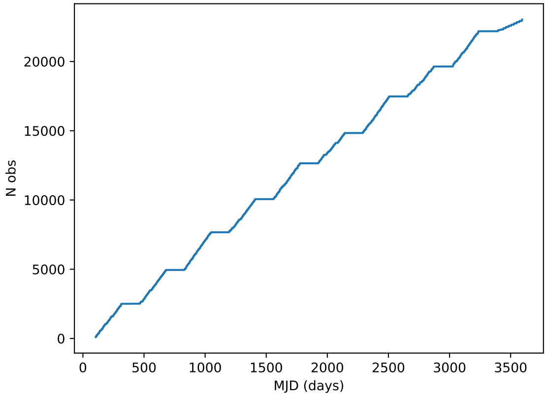
early_ss_template_fpextra5.0_v3.4_10yrs all bands: DD:EDFS Cumulative NVisits
