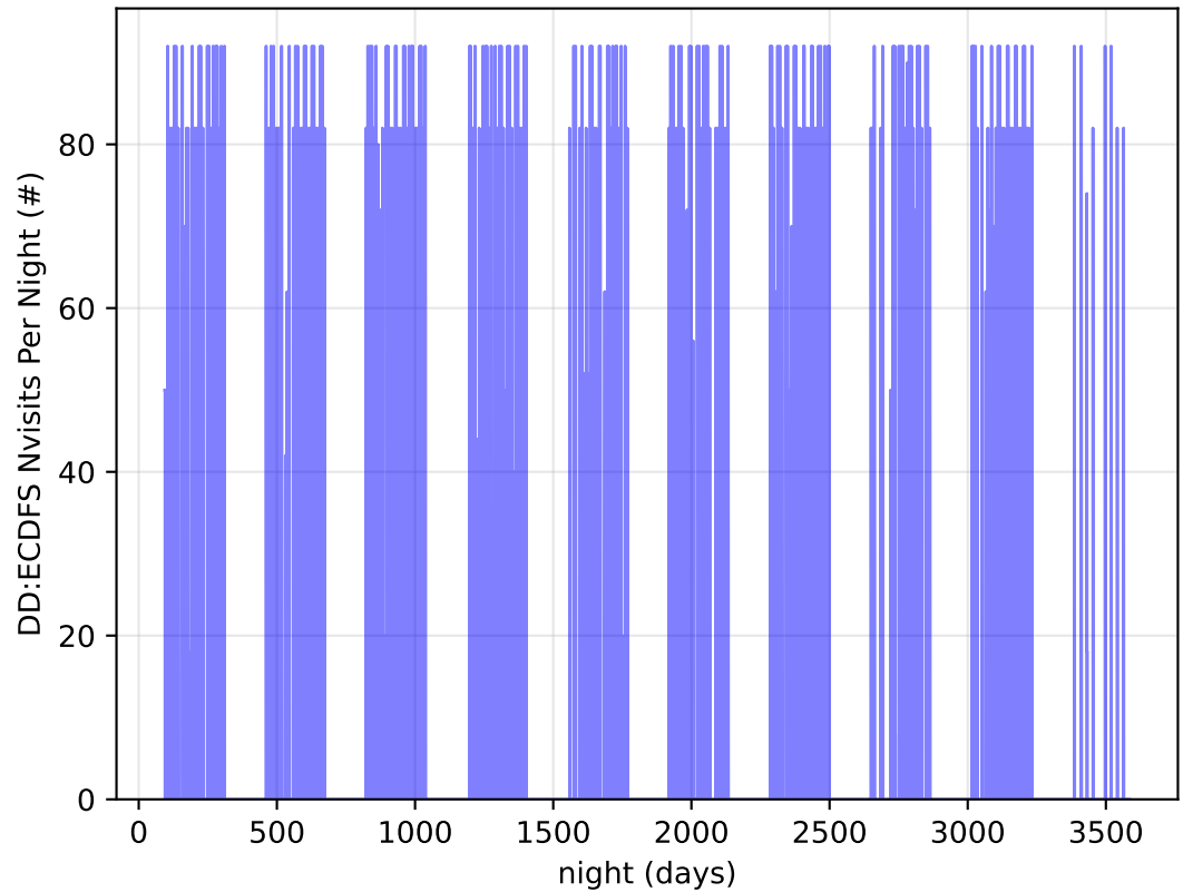
early_ss_template_fpextra5.0_v3.4_10yrs all bands: DD:ECDFS Nvisits Per Night
