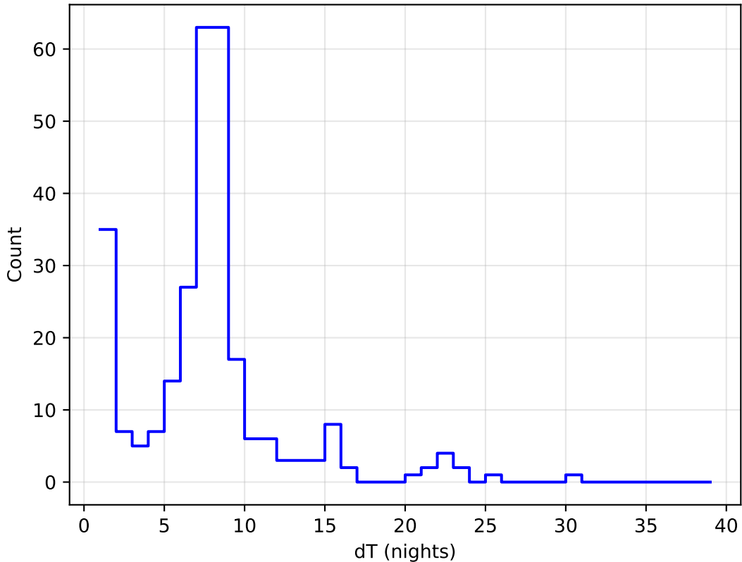
early_ss_template_fpextra5.0_v3.4_10yrs all bands: DD:ECDFS Delta Nights Histogram
