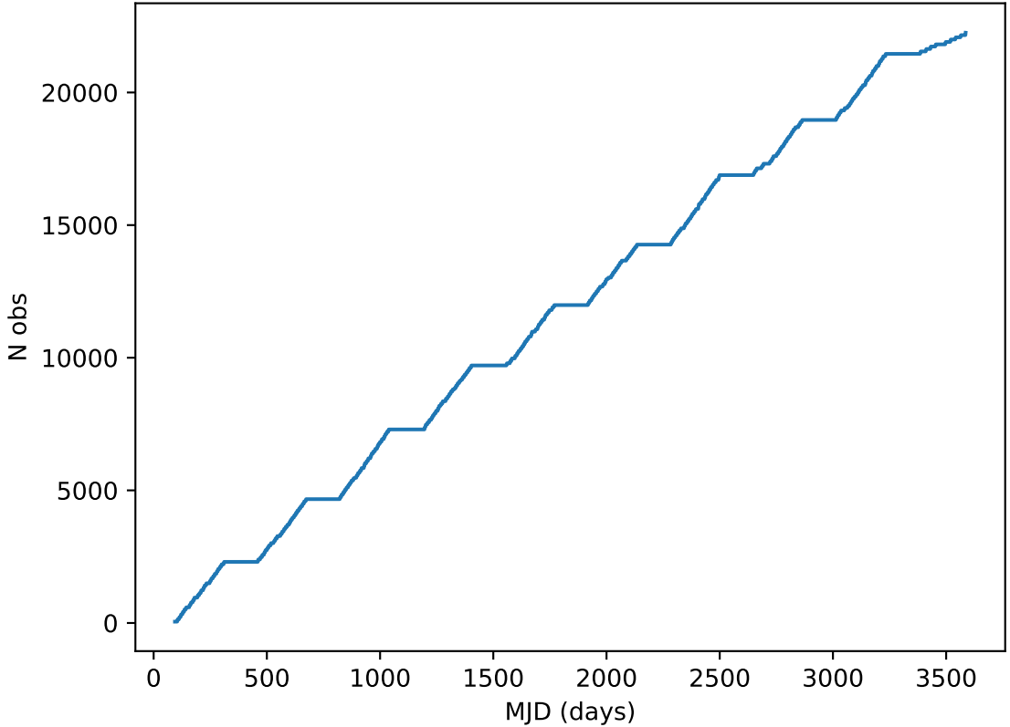
early_ss_template_fpextra5.0_v3.4_10yrs all bands: DD:ECDFS Cumulative NVisits
