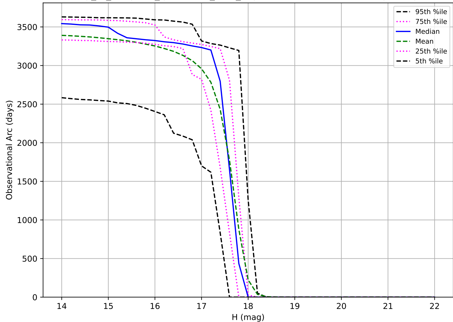
early_ss_template_fpextra3.0_v3.4_10yrs: Observational Arc Length Trojan
