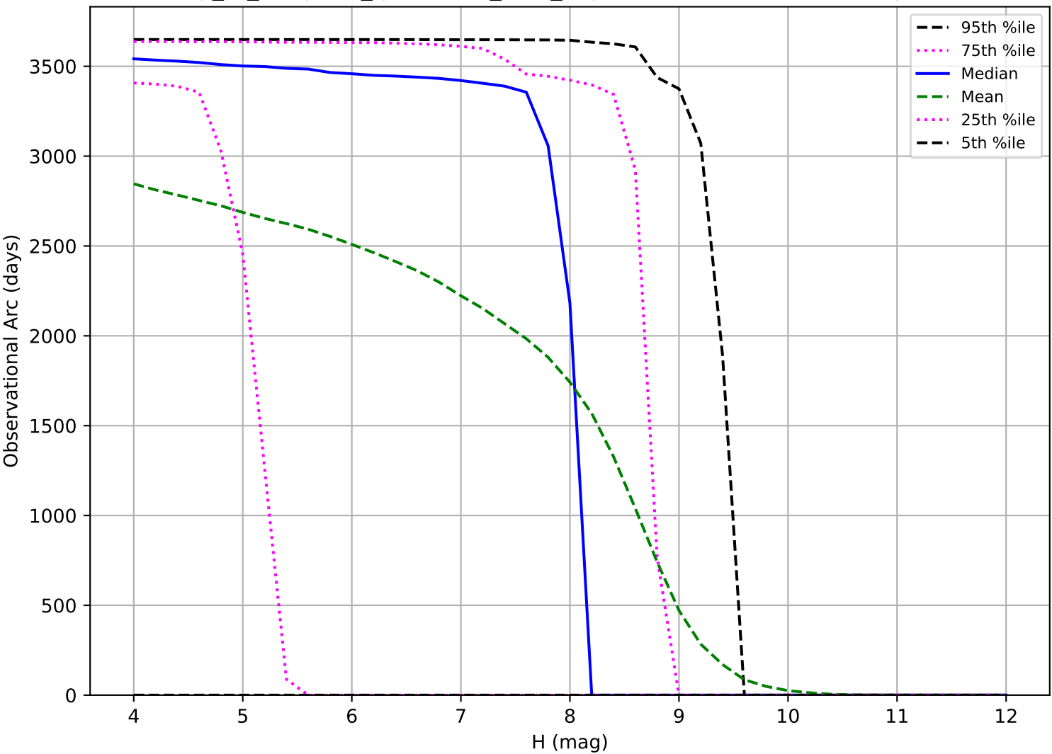
early_ss_template_fpextra3.0_v3.4_10yrs: Observational Arc Length TNO
