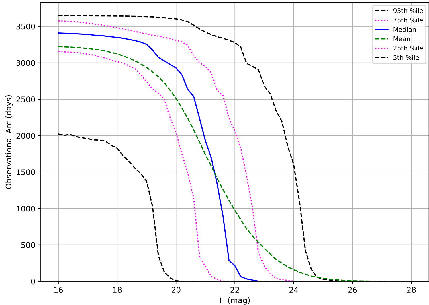
early_ss_template_fpextra3.0_v3.4_10yrs: Observational Arc Length PHA
